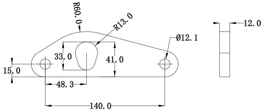
Standard 2: 360° rotating hook suspension assembly
