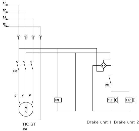
High voltage directly control-double brake-3ph
