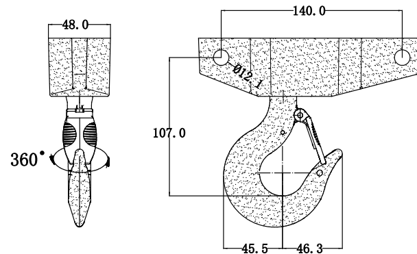
Standard 2: 360° rotating hook suspension assembly
