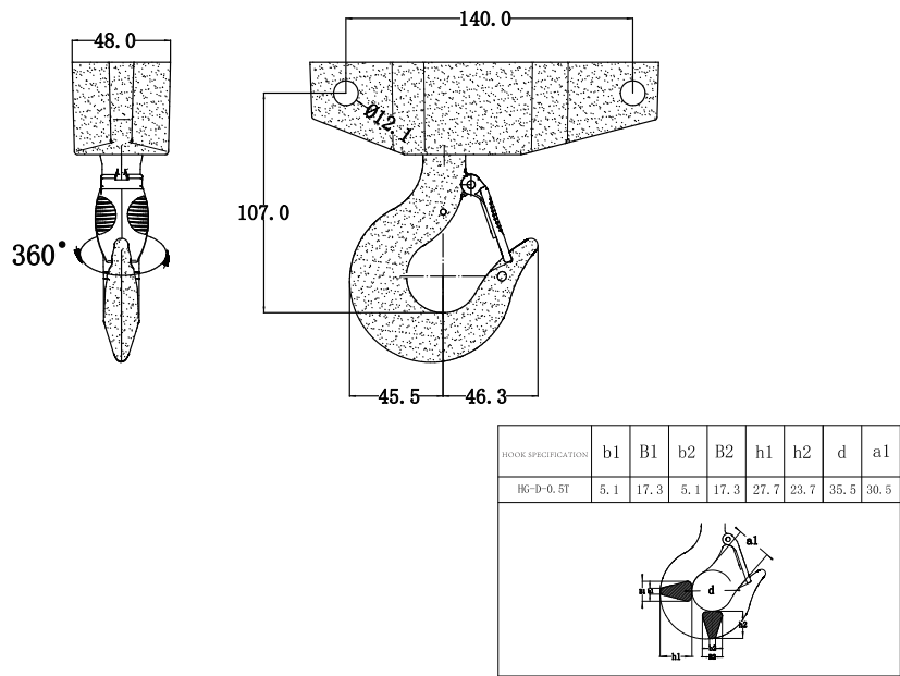
Standard 2: 360° rotating hook suspension assembly
