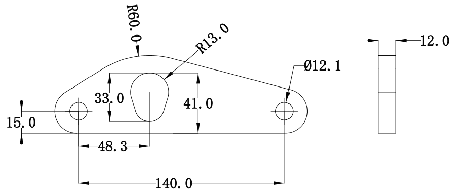
Standard 2: 360° rotating hook suspension assembly
