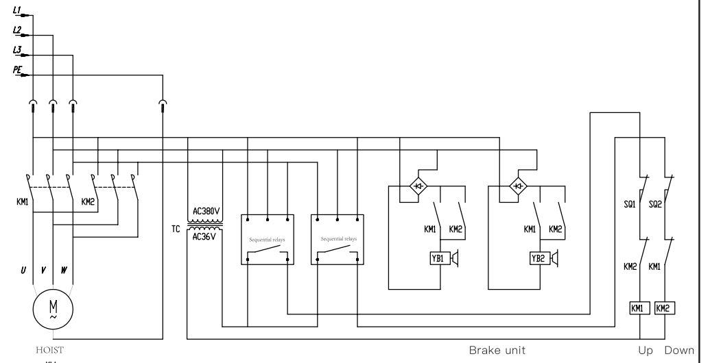
High voltage directly control-double brake-3ph
